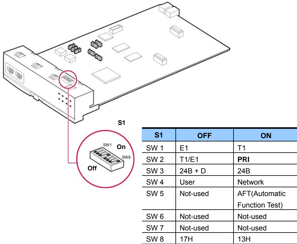
Figure 3.7 Setting the Switch of the TEPRI Board
