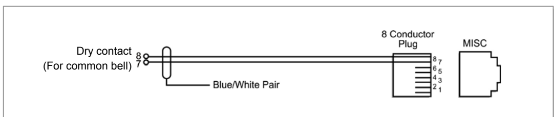
Figure 7.13 Connecting Common Bells
