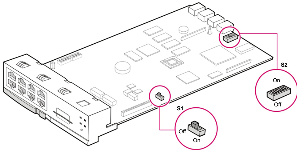
Figure 3.2 Setting Switches of MP10/11 Board
