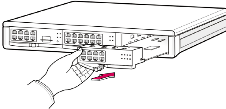
Figure 3.15 Replacing a New Board
