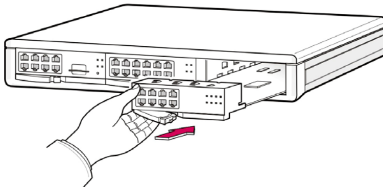
Figure 3.10 Mounting an Interface Board on a Slot
