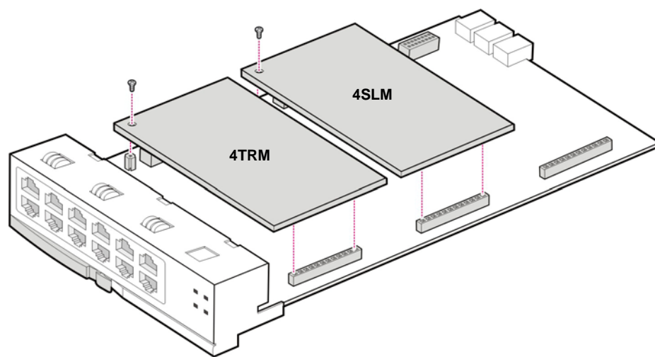
Figure 3.6 Mounting the UNI Board
