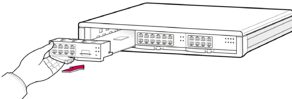
Figure 3.4 Mounting the Control Board to Slot 0
