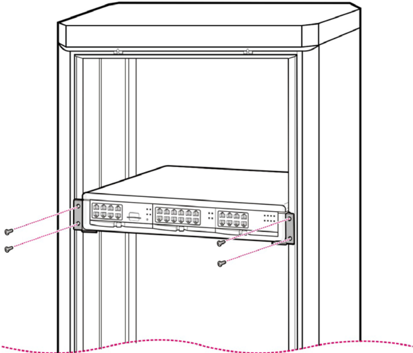
Figure 2.4 Rack Installation (3)
