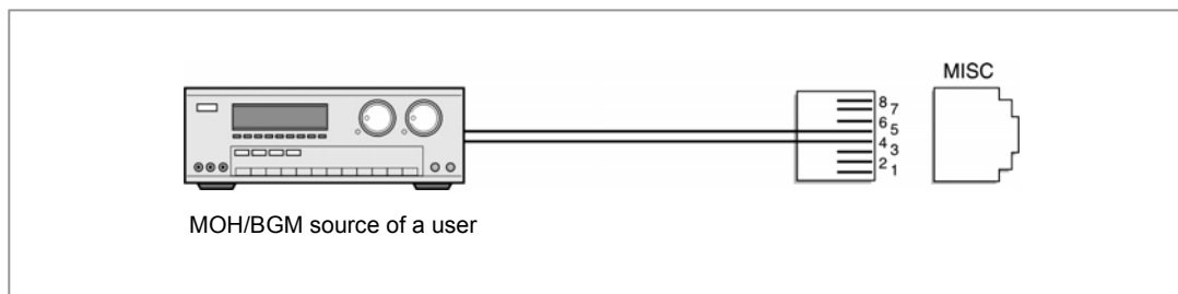
Figure 7.11 Connecting MOH/BGM Sources
