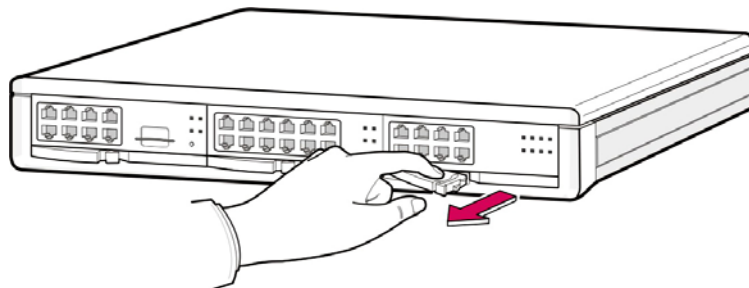
Figure 3.14 Removing a Board
