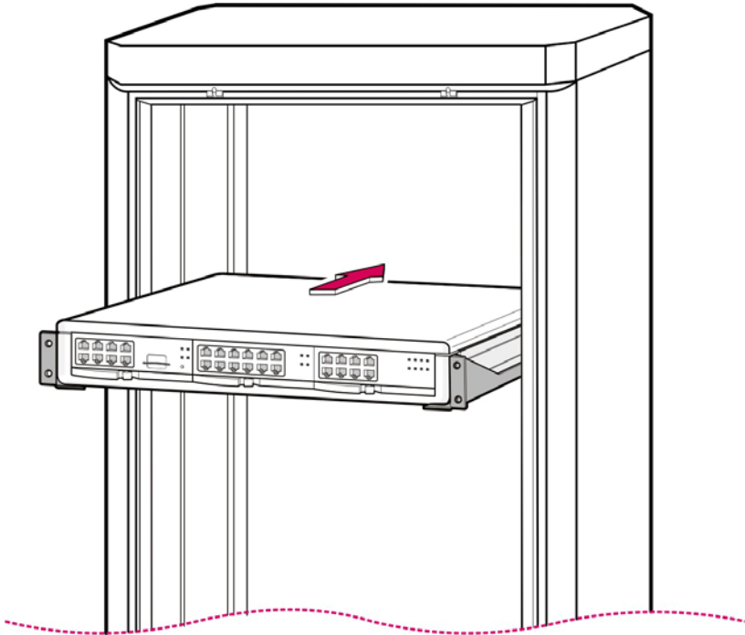
Figure 2.3 Rack Installation (2)
