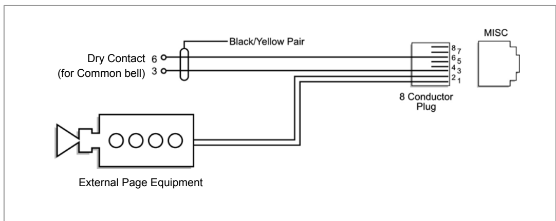
Figure 7.12 Connecting External/Additional Page Equipment
