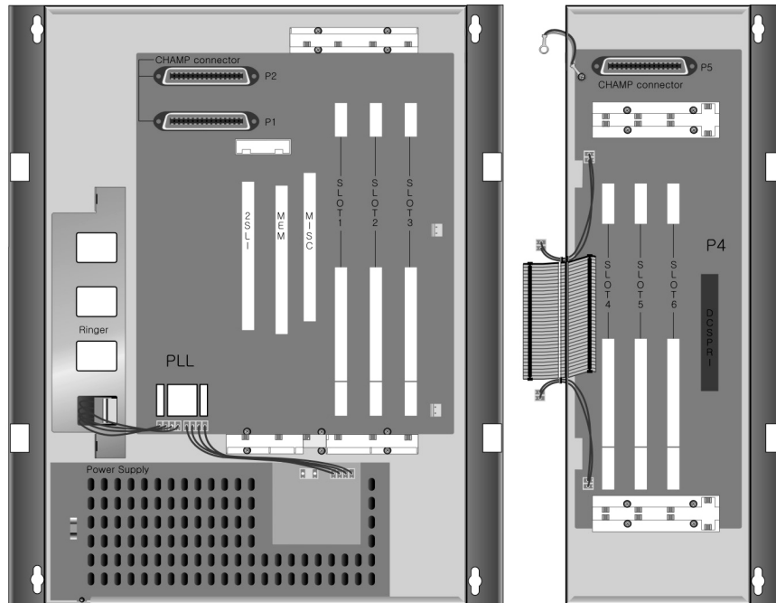
Figure 1.6 OfficeServ 100 System Configuration (Basic KSU + Expansion A)
