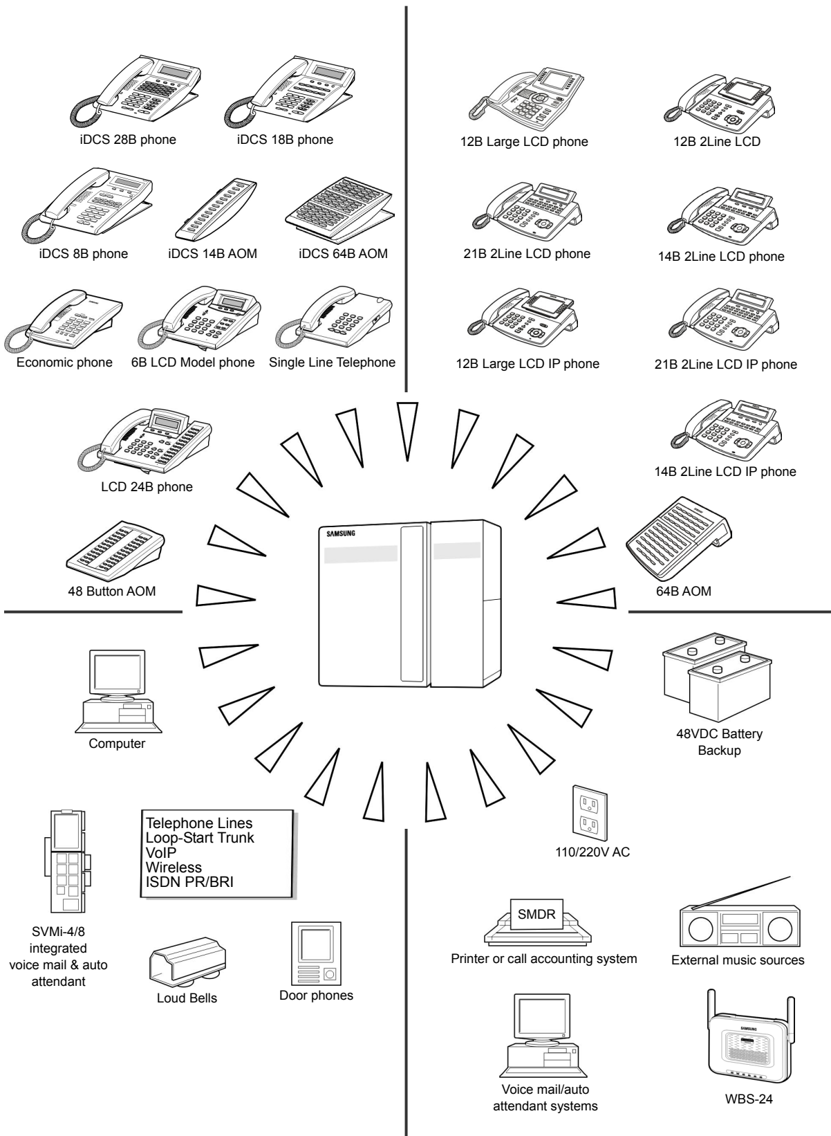
Figure 1.1 OfficeServ 100 General System Diagram
