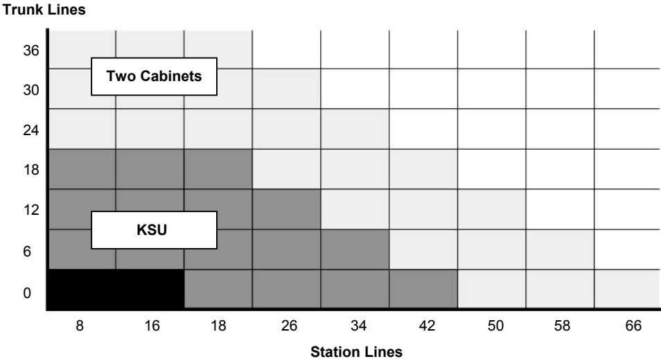
Figure 1.2 OfficeServ 100 Configuration Matrix Table (with Analogue Trunks)-Expansion A type
